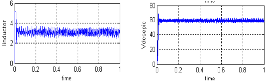
Fig 7: Inductor Current ( I_{l1} ) and Output Voltage of SEPIC Converter
