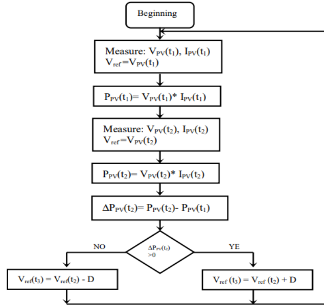
Fig 2: P&O algorithm
