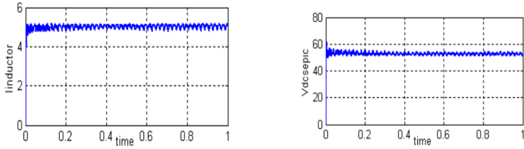
Fig 8: Inductor Current ( I_{l1} ) and Output Voltage of SEPIC Converter
